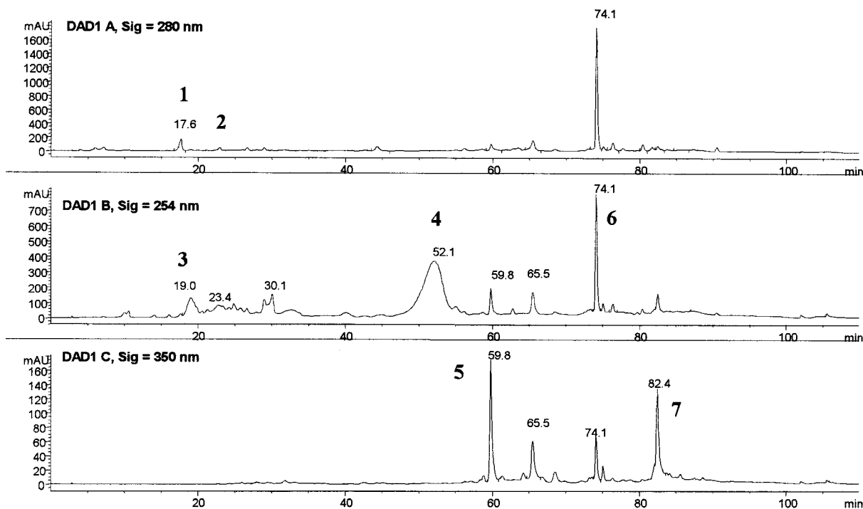
Figure 2. Chromatographic profiles of French ExpOOWW at 280, 254, and 360 nm. Peaks: 1, hydroxytyrosol; 2, tyrosol; 3, elenolic acid derivative; 4, elenolic acid; 5, luteolin 7- O -glucoside; 6, cinnamic acid derivative; 7, luteolin.
